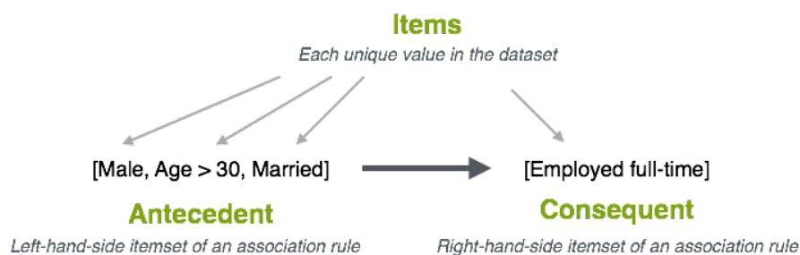
Figure 5.1: Association rule example
