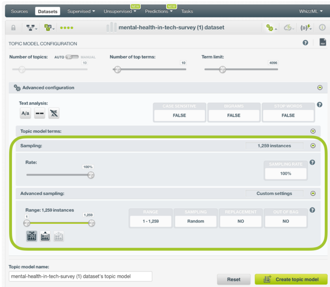
Figure 4.13: Sampling options for topic models
