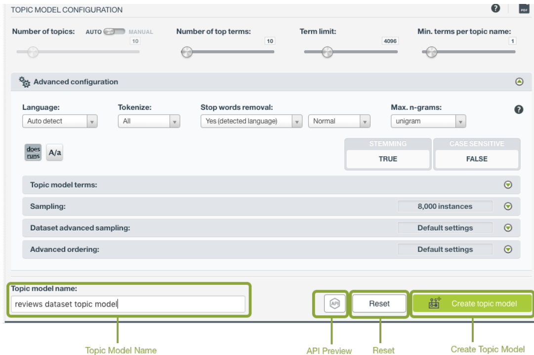
Figure 4.14: Create topic model after configuration
