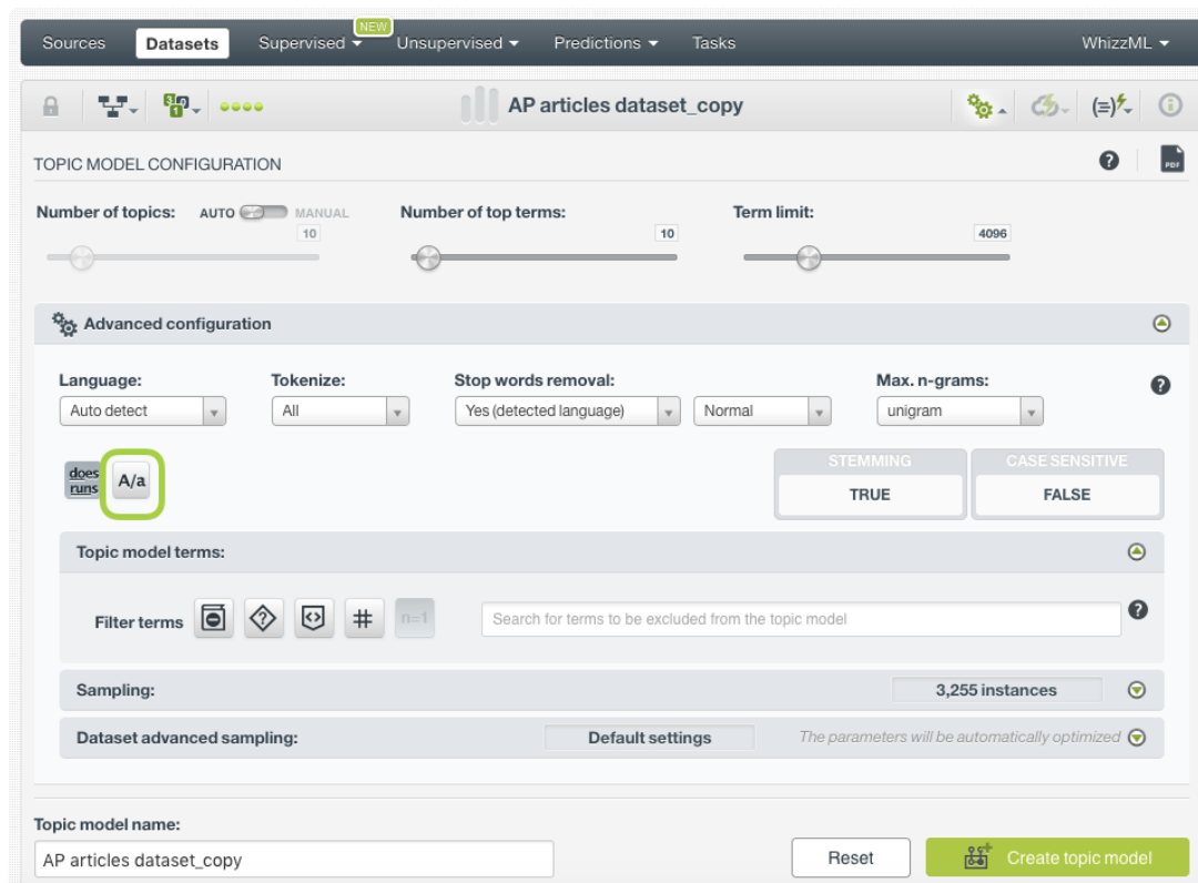
Figure 4.11: Case sensitivity configuration
