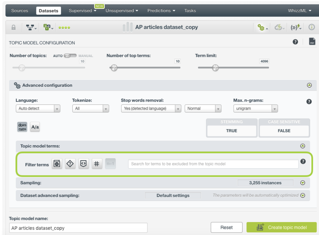
Figure 4.12: Filter terms
