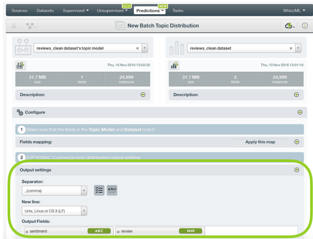
Figure 6.20: Output file settings for batch topic distributions
