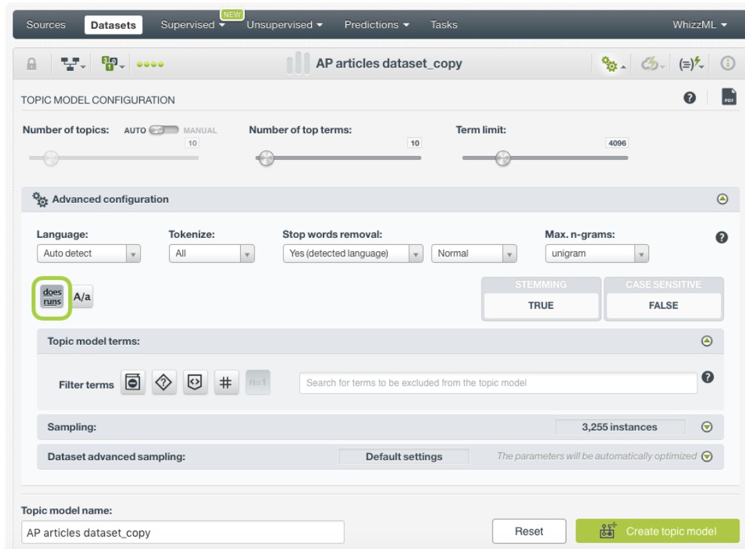
Figure 4.10: Stemming configuration
